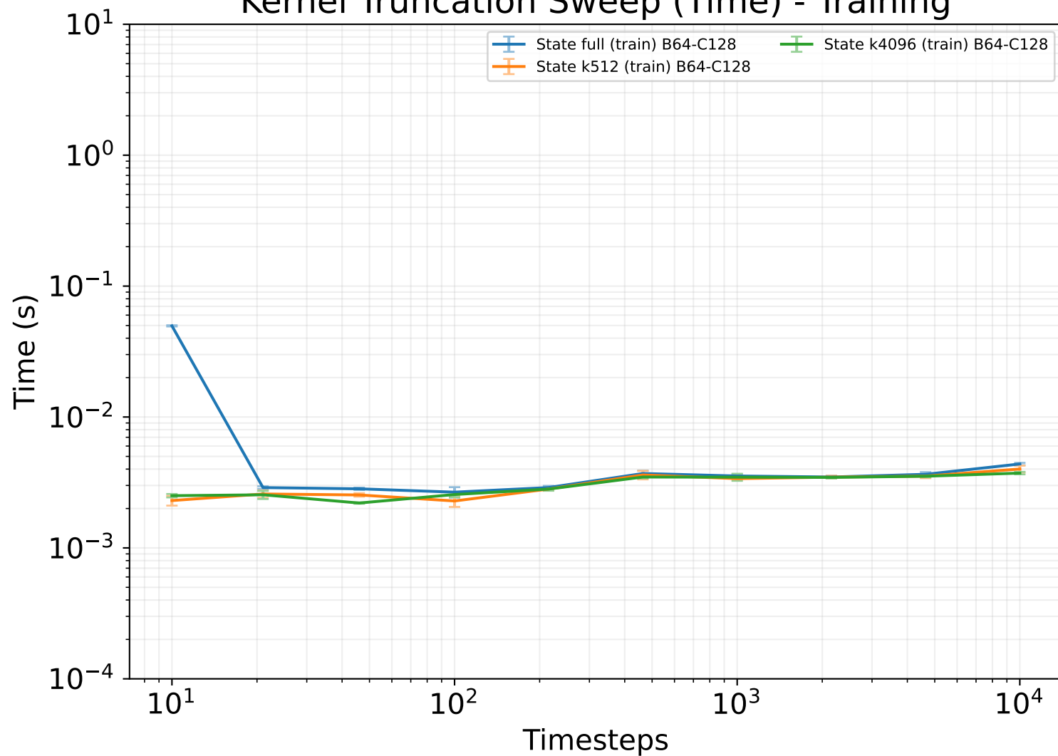
Kernel Truncation Sweep (Time) - Training
